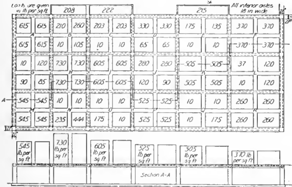
FIG. 2. DIAGRAM OF FINAL LOAD
